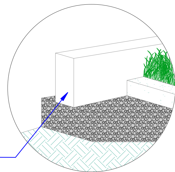
BENDER BOARD OR METAL EDGING (NOT SUPPLIED)
